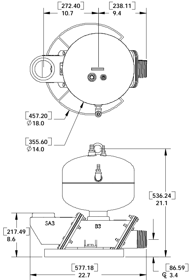
All dimensions in inches [millimeters]
