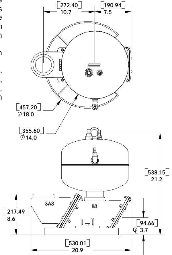
All dimensions in inches [millimeters]
